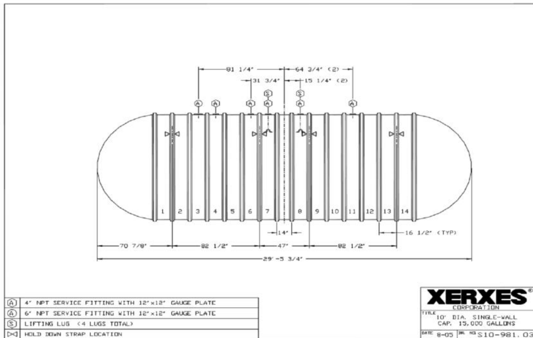
Fig. 7.2 Above Storage Tank for Diesel Fuel
