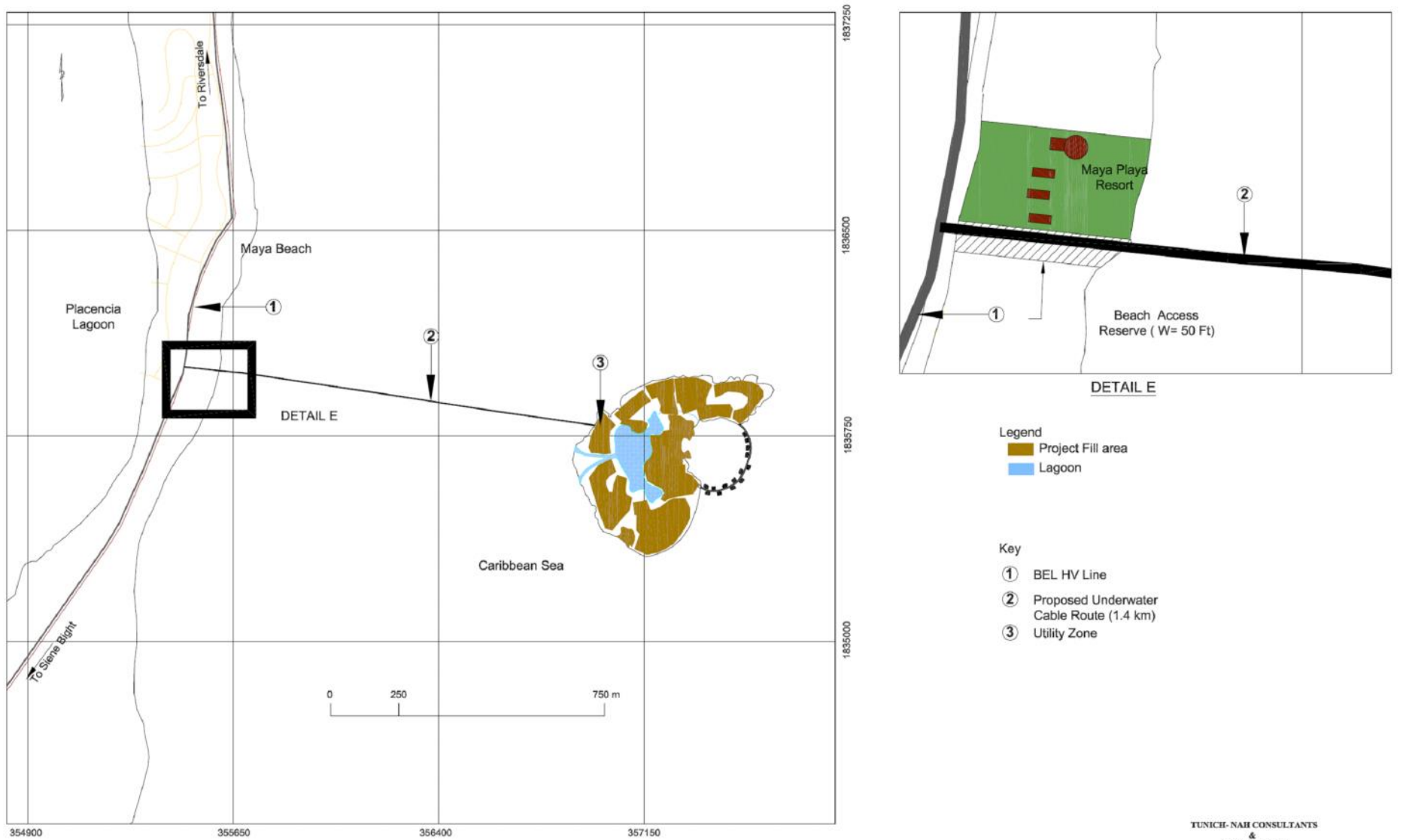
Fig. 7.1 Proposed BEL HV Line Underwater Route
